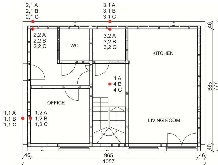
Fig. 2. Location of temperature measurement sections (dimensions in cm)
