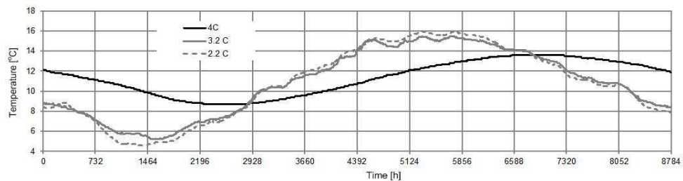
Fig. 6. Measured, yearly temperature pattern at the bottom of thermal insulation (measurement points location shown on Fig. 2, 3)
