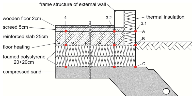
Fig. 3. Vertical section of foundation interface with measurement points
