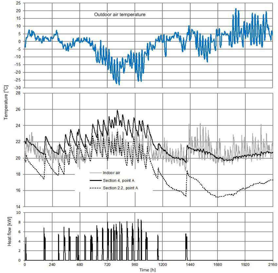
Fig. 5. Pattern of outdoor (top diagram) and indoor temperature, temperature measured at points 4A, 2.2A (lower diagram), and heat supply to floor, 1 st Jan. – 30 th March, 2012 (measurement points location shown on Fig. 2, 3)
