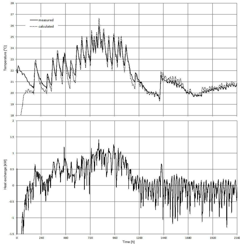
Fig. 7. Measured and calculated temperature pattern at section 4, point A (measurement points location shown on Fig. 2, 3) and total heat exchange between inner air and floor, 1 st January – 30 th March, 2012
