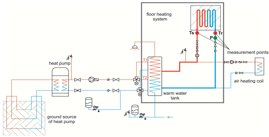
Fig. 4. Heating system with measurement points of supply ( T_s ), return temperature ( T_r ) and water flow ( P ) for floor heating
